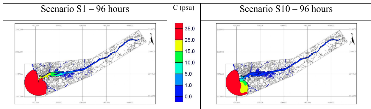
Fig. 9 Mass transport model: salinity concentration gradient for the adopted extreme river discharges.
