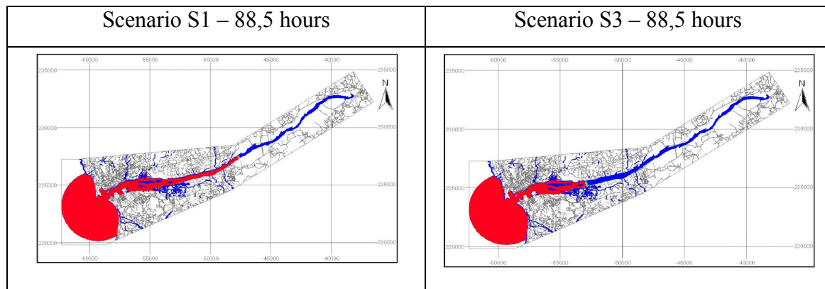
Fig. 8 Mass transport model: intrusion extent for different tidal conditions.
