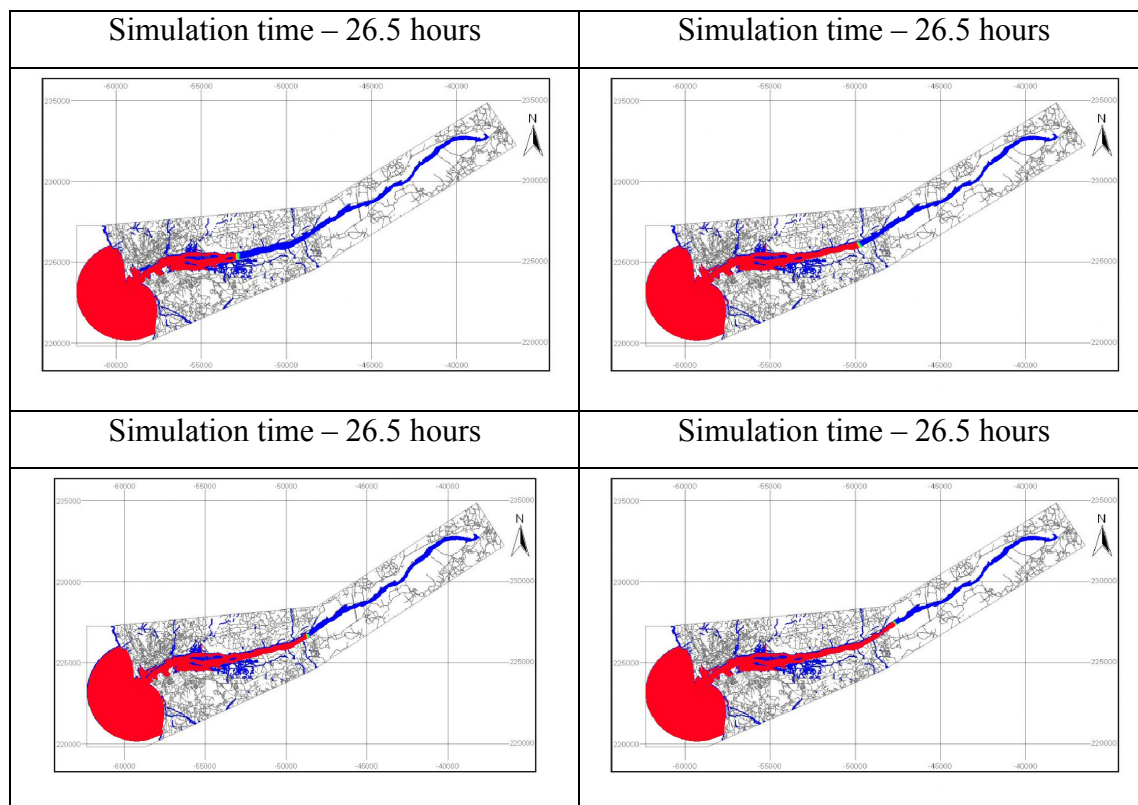
Fig. 7 Mass transport model: intrusion extent for successive tide flood events (S1).
